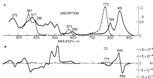
Figure 4. Spectra of BChl a in diethyl ether solution (dashed curves) and of chromatophores of the photosynthetic bacterium Rhodospseudomonas spheroides , wild type (solid curves). (A) Absorption spectra. (B) Circular dichroism. Path lengths, 1 cm.
